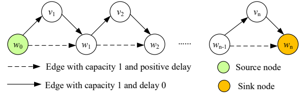
Fig. 1. Reduced network graph from partition problem.
