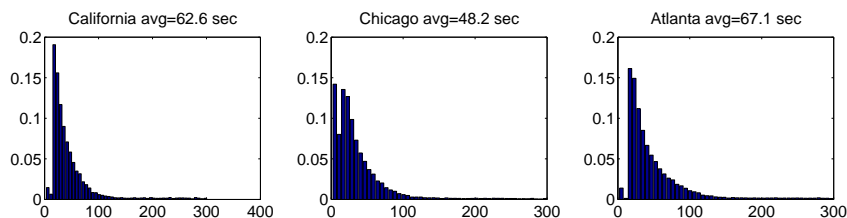
Figure 3: Distribution of Stop Length
