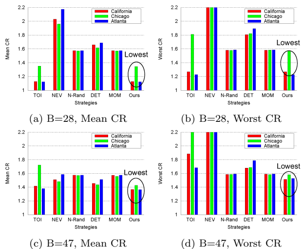
Figure 4: Individual Vehicle Test
