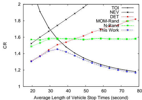
Figure 5: Worst case CR under different average stop lengths ( B = 28 )
