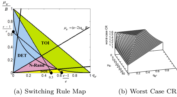
Figure 1: The Proposed Online Algorithm and its Worst Case CR
