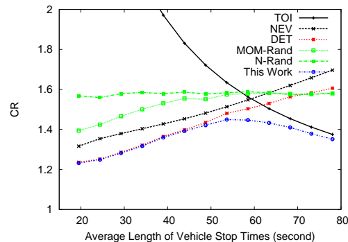
Figure 6: Worst case CR under different average stop lengths ( B = 47 )
